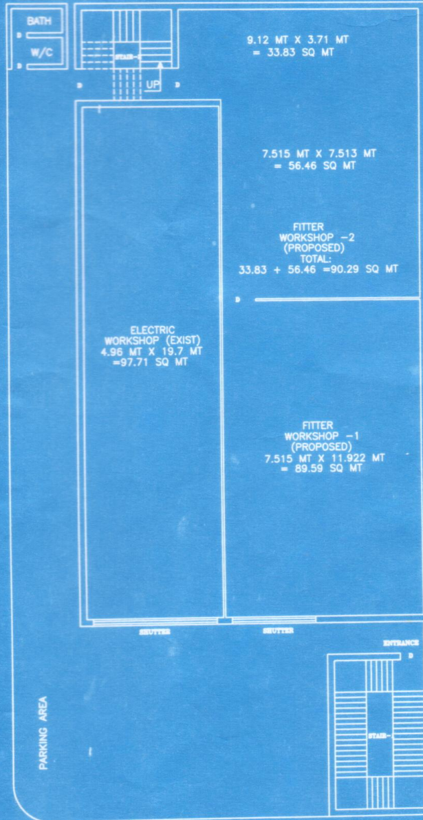
GROUND FLOOR PLAN OF I.T.I.
