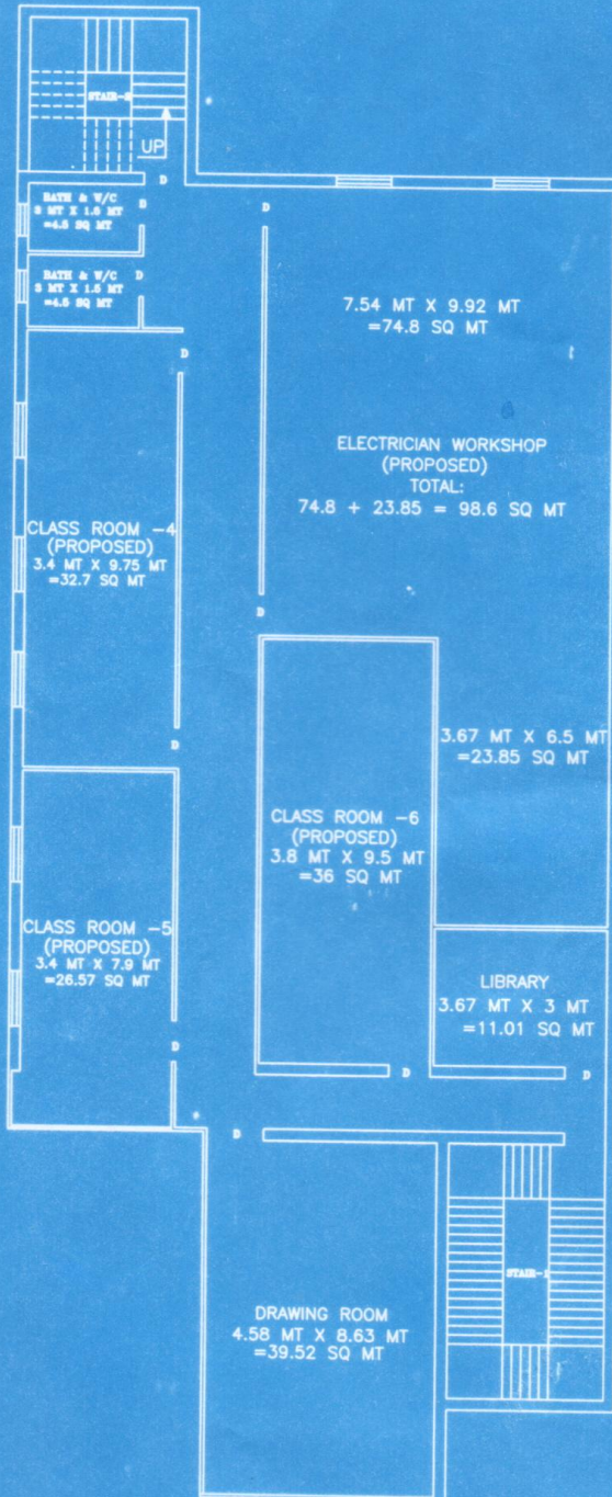
THIRD FLOOR PLAN OF I.T.I.
